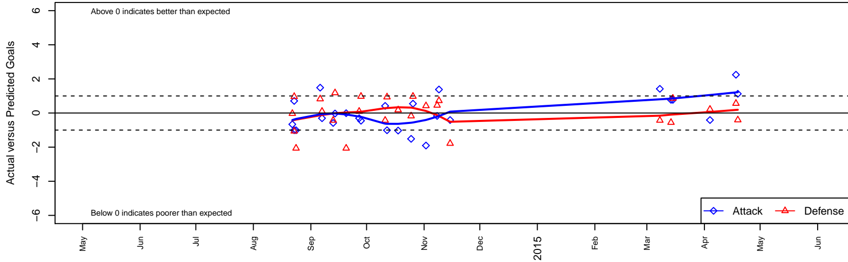
TFA Barcelona OR G03 Dots are actual minus expected GF (blue circles) and GA (red triangles). Blue line is smoothed change in attack strength. Red is smoothed change in defense strength.
